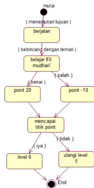
Gambar 3.5. FSM Game Level 5
