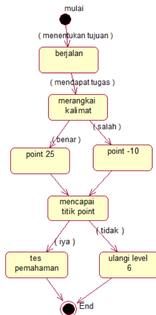
Gambar 3.6. FSM Game Level 6
