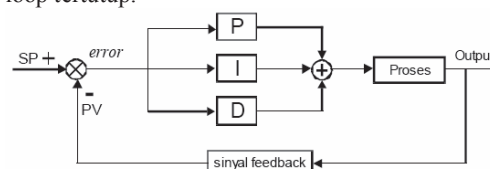
Gambar 1 Blok Diagram PID controller Loop Tertutup
