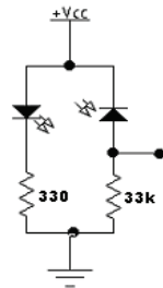
Gambar 3 Rangkaian Sensor Garis Sumber: (Modul Line Tracer - MC Teknik Elektro ITS, 2004)
