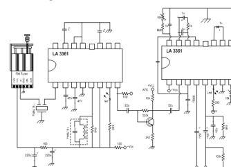
Gambar 6 Rangkaian Penerima FM straight
