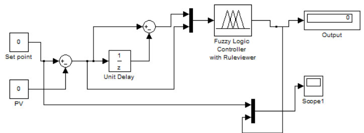
Figure 3.1 Fuzzy Control
